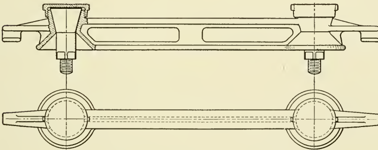
Fig. 1. Double Trolley Insulator Used in the Schiemann System
